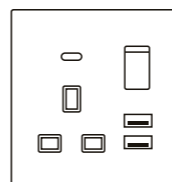
E-045 13A switched socket+2USB w/without neon(single pole)
