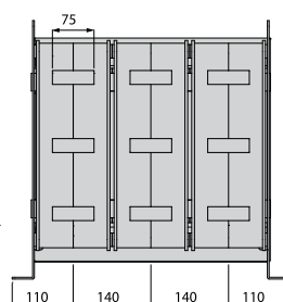
2000~2500A Back View
