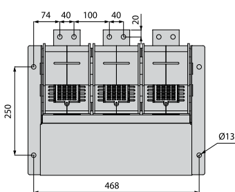
2000~2500A Bottom View
