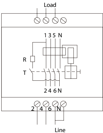
For Three Phase - 3 Wire
