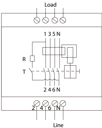
For Three Phase - 4 Wire
